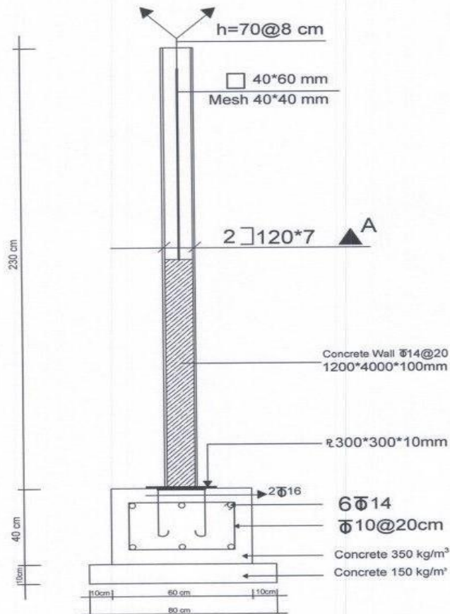
Iran touring & tourism investment company Sorkhrood resort complex (Wall section)
